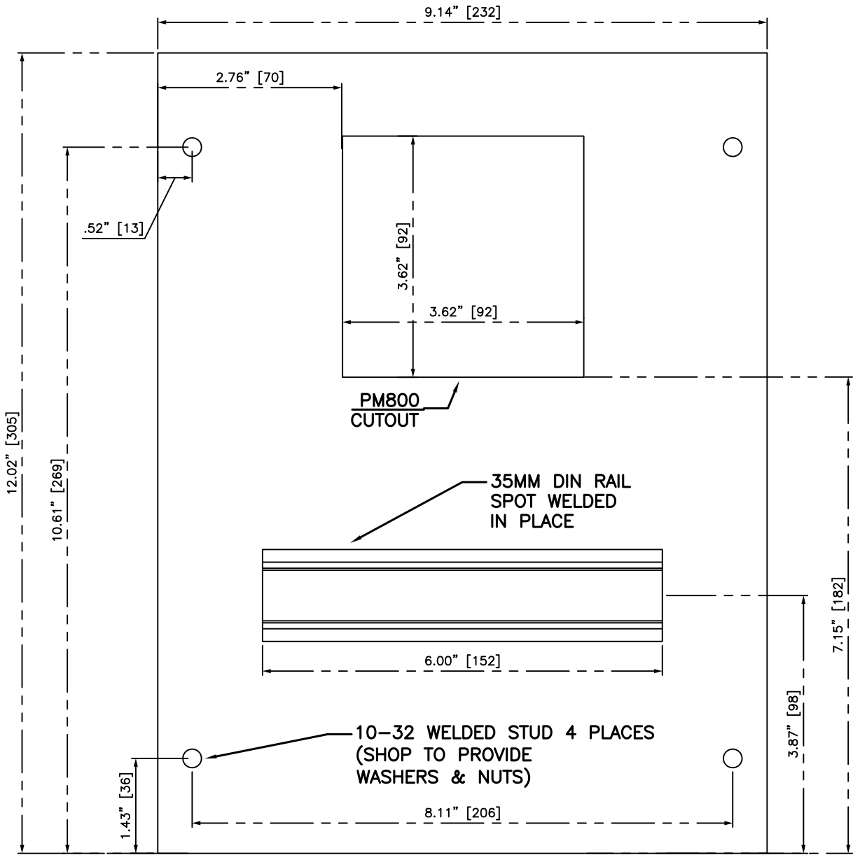
FRONT PLATE REAR VIEW
