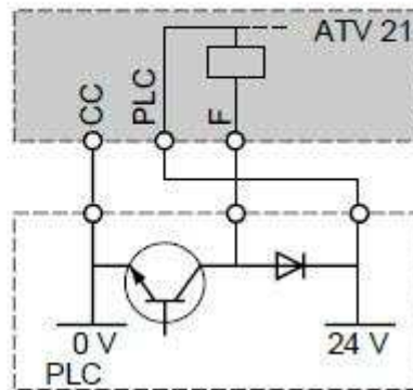
Sinking PLC
