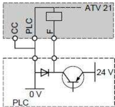
Sourcing PLC
